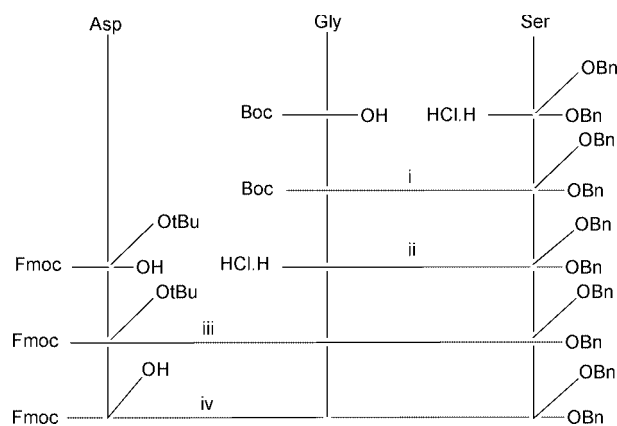
Scheme 4 Reagents and conditions: i, DPPA, Et 3 N, 0 °C → rt, 15 h (83%); ii, HCl 4 M-dioxane, 0 °C, 3 h; iii, DPPA-Et 3 N, 0 °C → rt, 15 h (59%); iv, TFA, rt, 2 h (90%).
