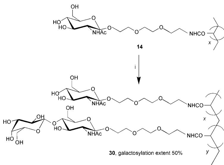
Scheme 7 Reagents and conditions: i, UDP-Gal (3 equiv. for 12 and 14 , 1.3 equiv. for 13 ), \alpha -lactalbumin (0.2 g dm -3 ), \beta -(1,4)-galactosyl transferase (1 U), HEPES buffer (pH 6.5, 50 mM, 1 cm 3 ), 37 °C, 72 h.
