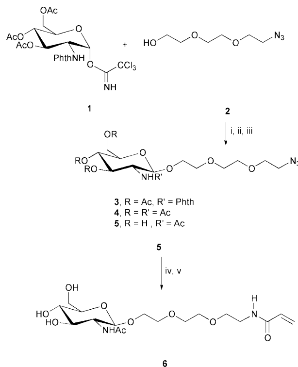
Scheme 1 Reagents and conditions: i, \text{BF}_3 \cdot \text{Et}_2\text{O} , 4 Å molecular sieves, \text{CH}_2\text{Cl}_2 , 0 °C → rt, 24 h; ii, ethylenediamine, n -butanol, 70 °C, 24 h then pyridine– \text{Ac}_2\text{O} , rt, 24 h; iii, MeONa, MeOH, rt, 2 h; iv, \text{H}_2 , Pd–C, MeOH, rt, 4 h; v, \text{CH}_2=\text{CHCOCl} , triethylamine, MeOH, 0 °C, 3 h.
