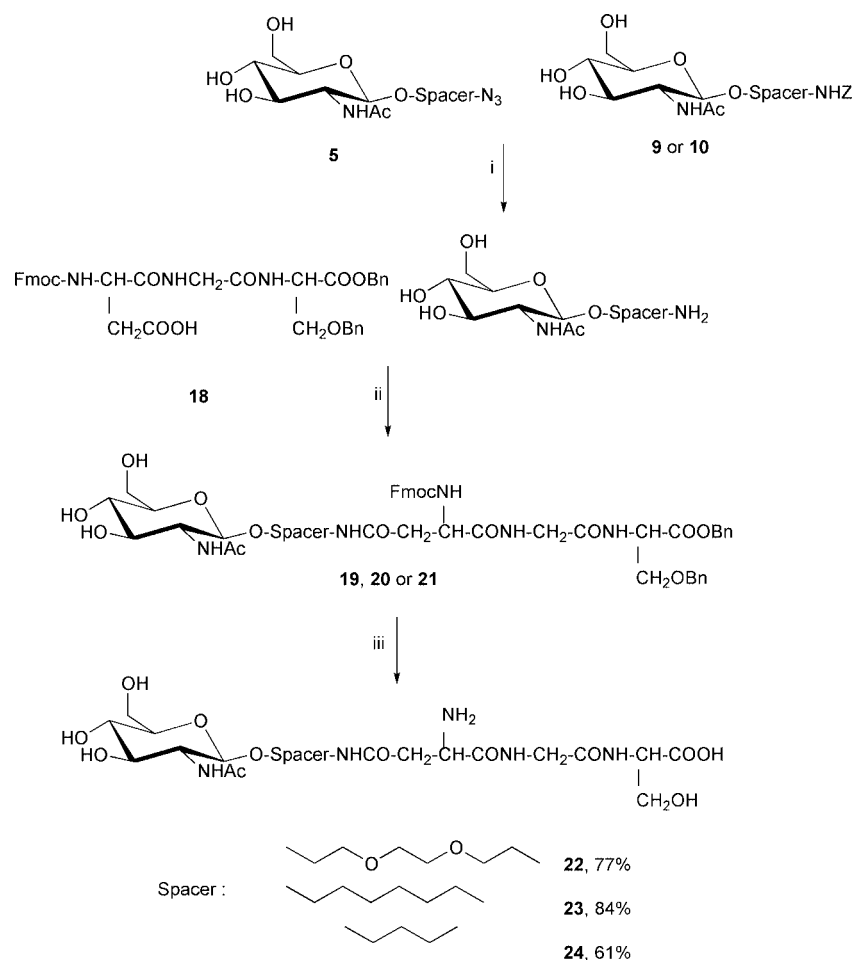
Scheme 5 Reagents and conditions: i, \text{H}_2 , Pd-C, MeOH, rt, 4 h (for 5 ) or \text{H}_2 , Pd-C, MeOH- \text{AcOH}_{\text{cat}} , rt, 3 h (for 9 and 10 ); ii, EEDQ, ethanol-benzene (1 : 1), rt, 24 h; iii, piperidine, DMF, 2 h, rt then \text{H}_2 , Pd-C, \text{AcOH-H}_2\text{O} (8 : 2), rt, 24 h.
