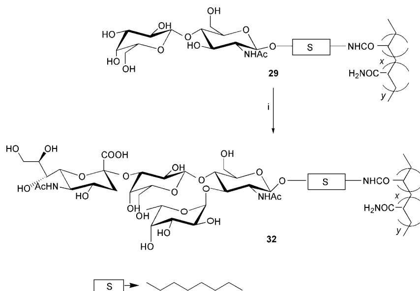
Scheme 8 Reagents and conditions: i, CMP-NANA (3 equiv.), \alpha -(2,3)-sialyl transferase (0.3 U), sodium cacodylate buffer (pH 6.0, 50 mM), 0.1% Triton X-100, 37 °C, 5 d. then GDP-Fucose (2 equiv.), \alpha -(1,3)-fucosyl transferase V (10 mU), HEPES buffer (pH 7.5, 100 mM), NaN 3 , MnCl 2 ·4H 2 O, 37 °C, 3 d.
